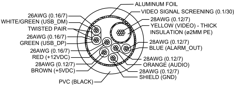
CABLE BUILDUP
